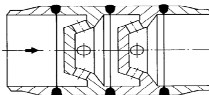
Figure 6 Multiport Throttle SSD 5
