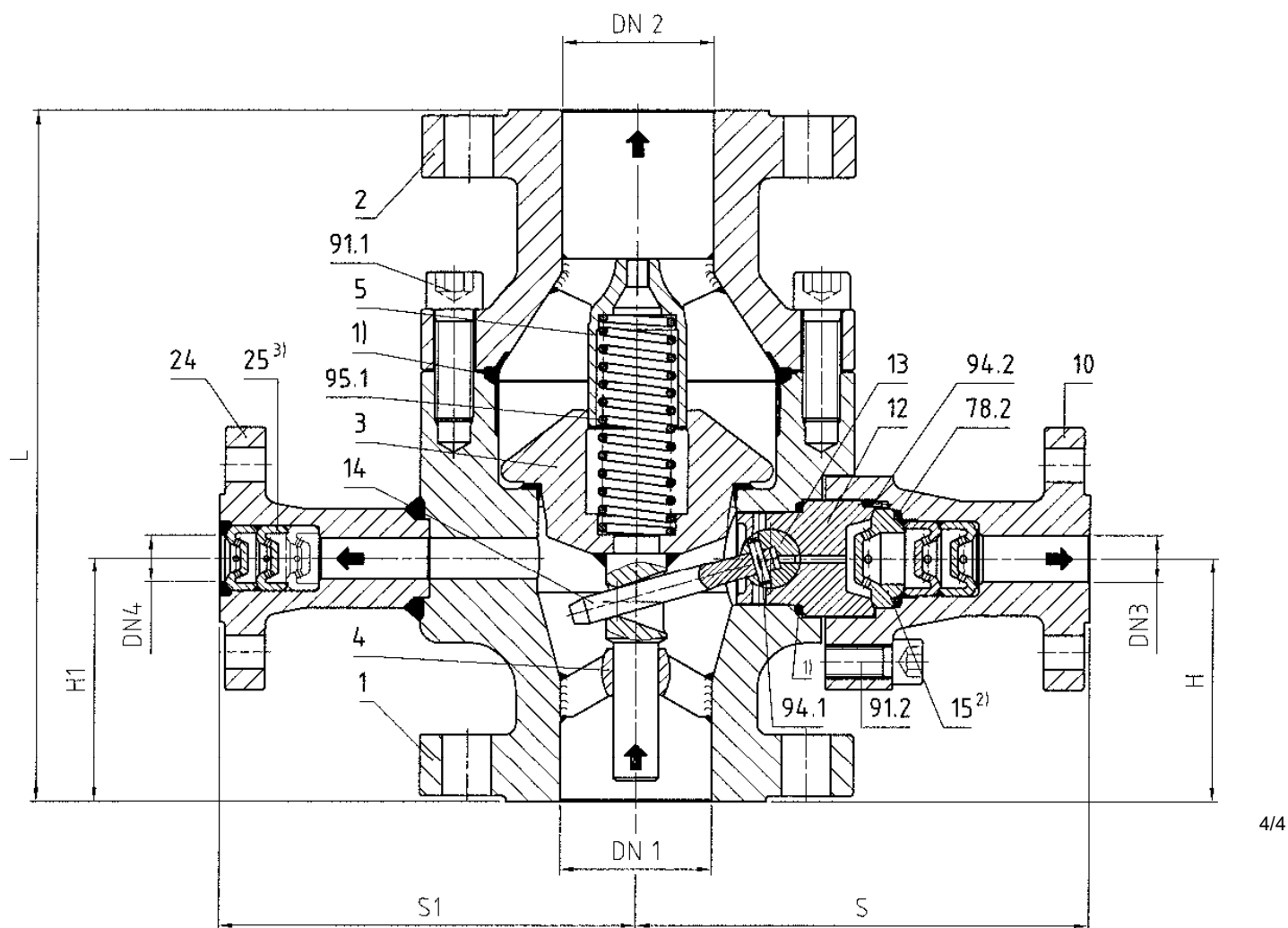
Figure 5 SSV 10/12 with multistage pressure and flow reduction in the bypass
